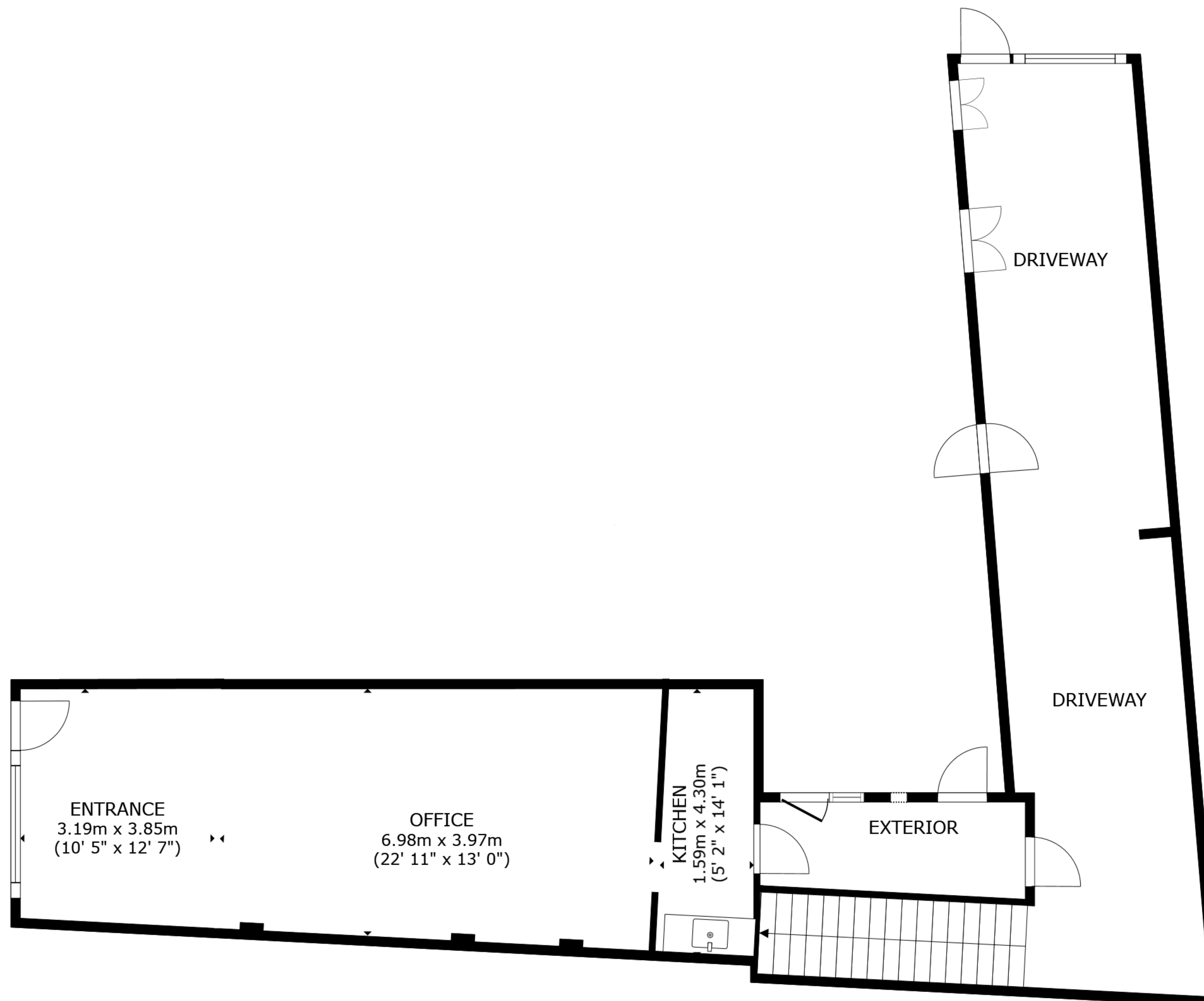
FLOOR PLAN
