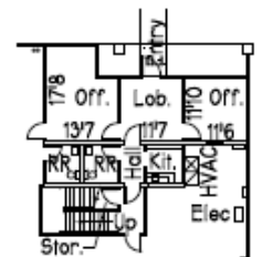
Ground Floor Plan 14532 Garfield Scale: 1" = 30'
