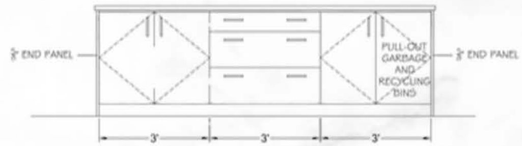
KITCHEN ISLAND - ELEVATION
