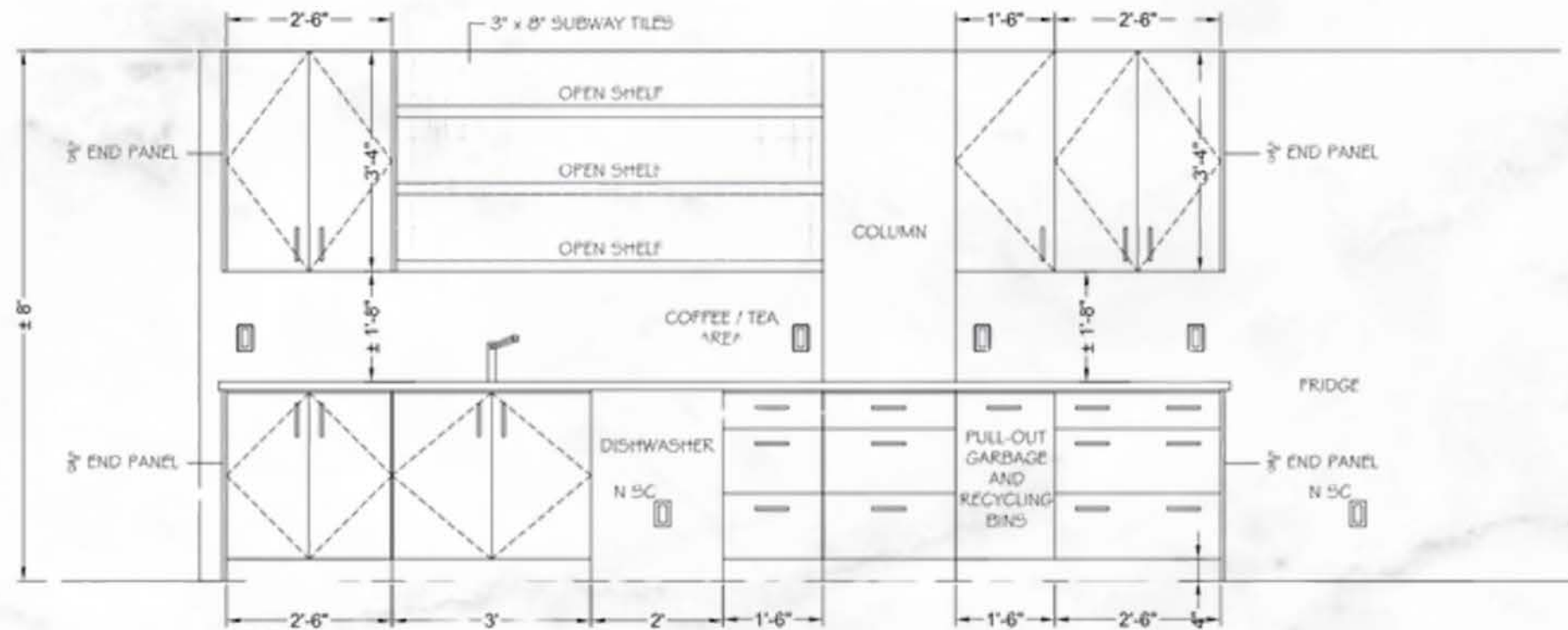
KITCHEN CABINETS - ELEVATION
