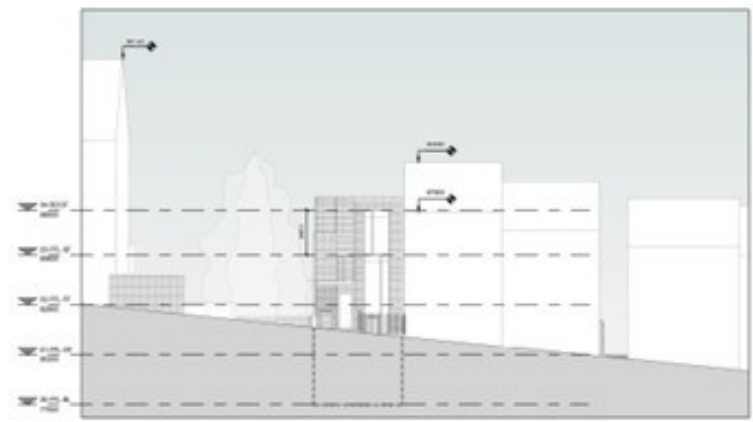
WEST ELEVATION 1 : 100
