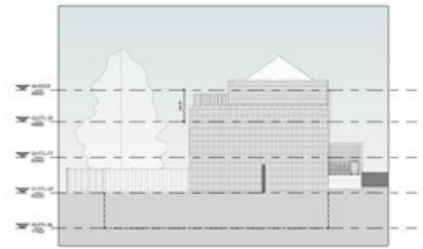
NORTH ELEVATION 1 : 100
