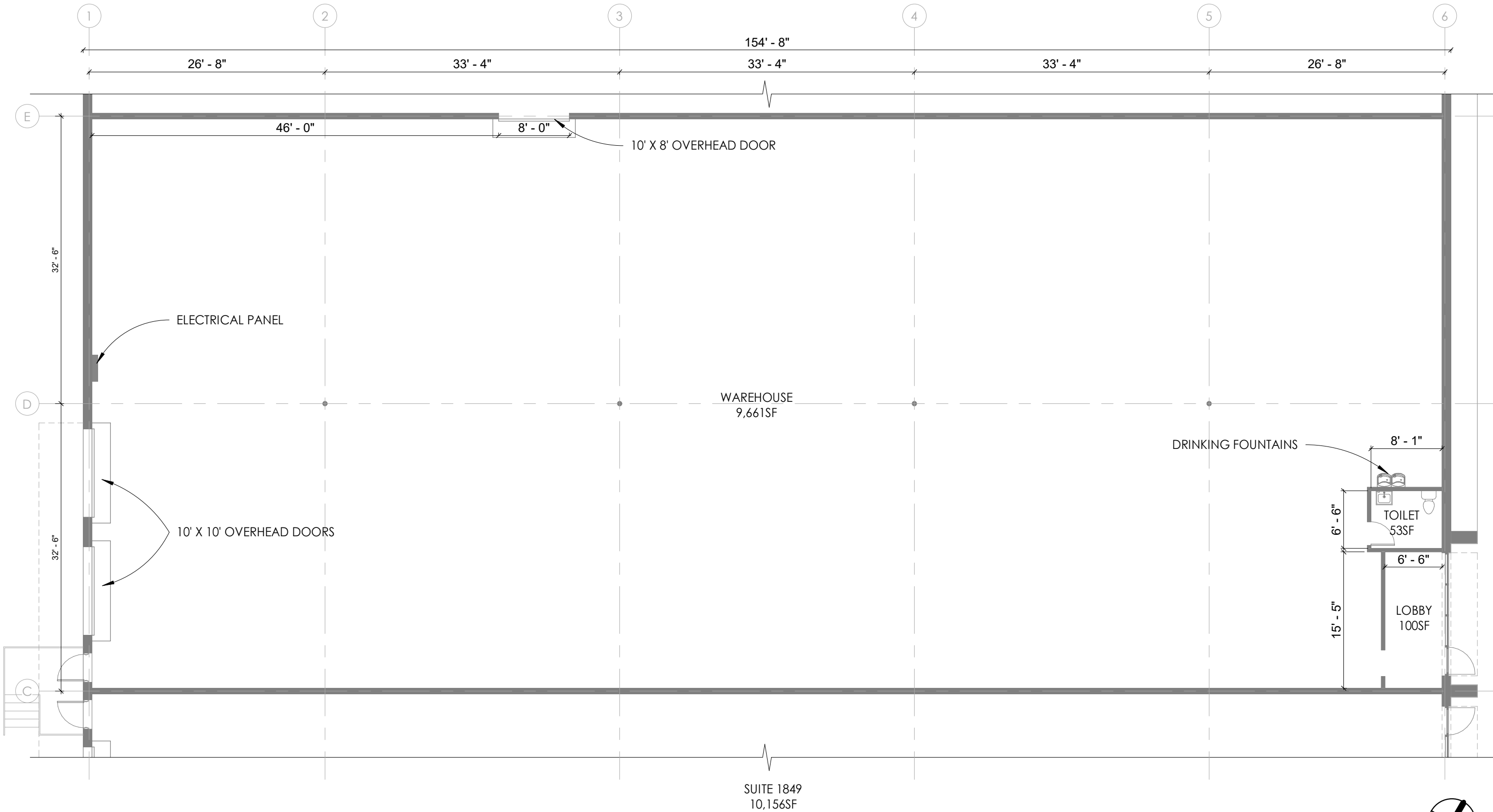
1 SUITE 1849 - EXISTING FLOOR PLAN 3/32" = 1'-0"
