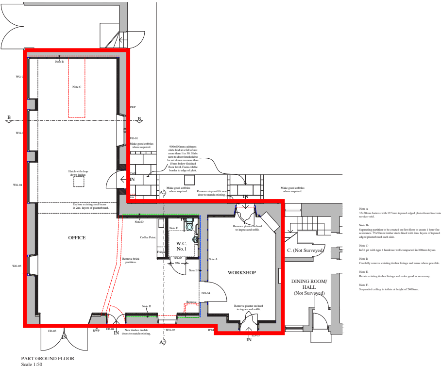
PART GROUND FLOOR Scale 1:50
