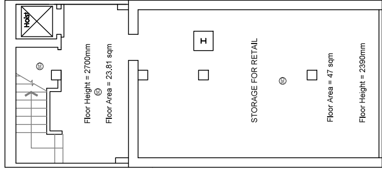
Proposed Basement Floor Plan Scale: 1:100
