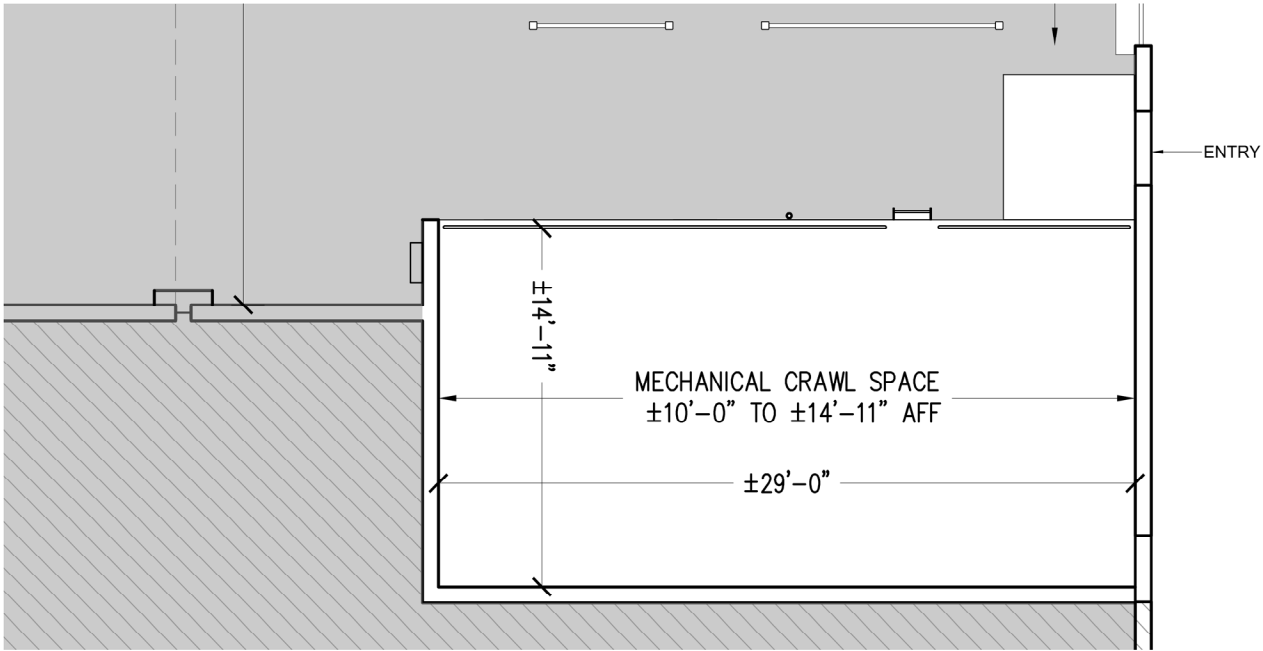
3 MECHANICAL LEVEL
