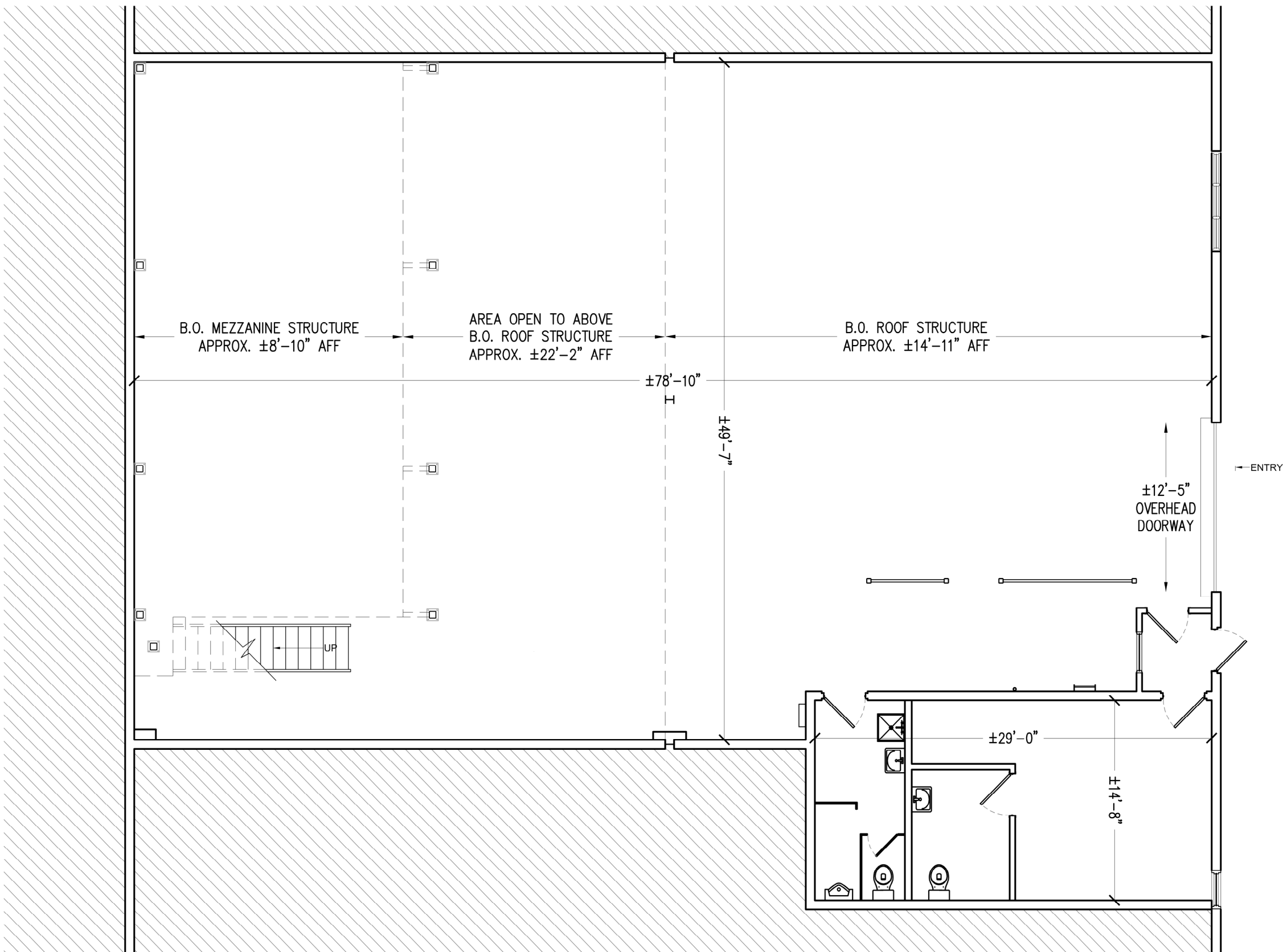
1 GROUND FLOOR
