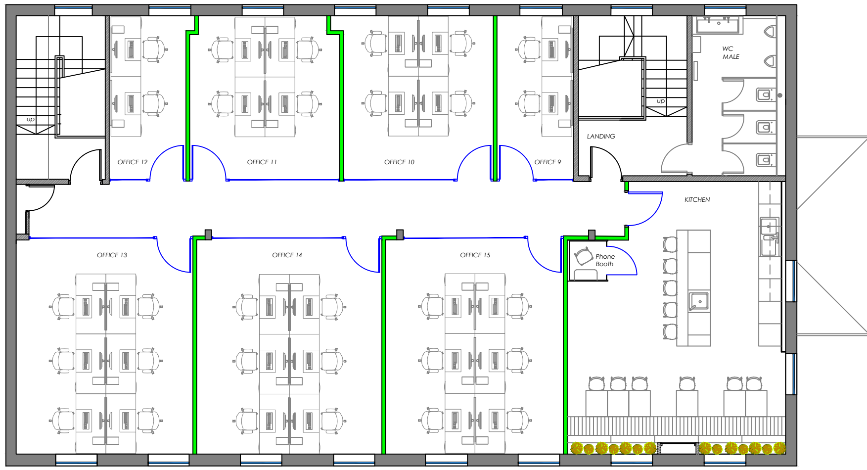
First Floor Plan As Proposed
