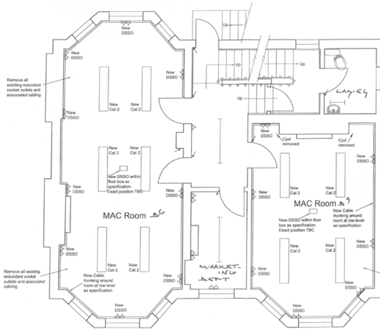
Cromwell Road Proposed First Floor Electrical Plan
