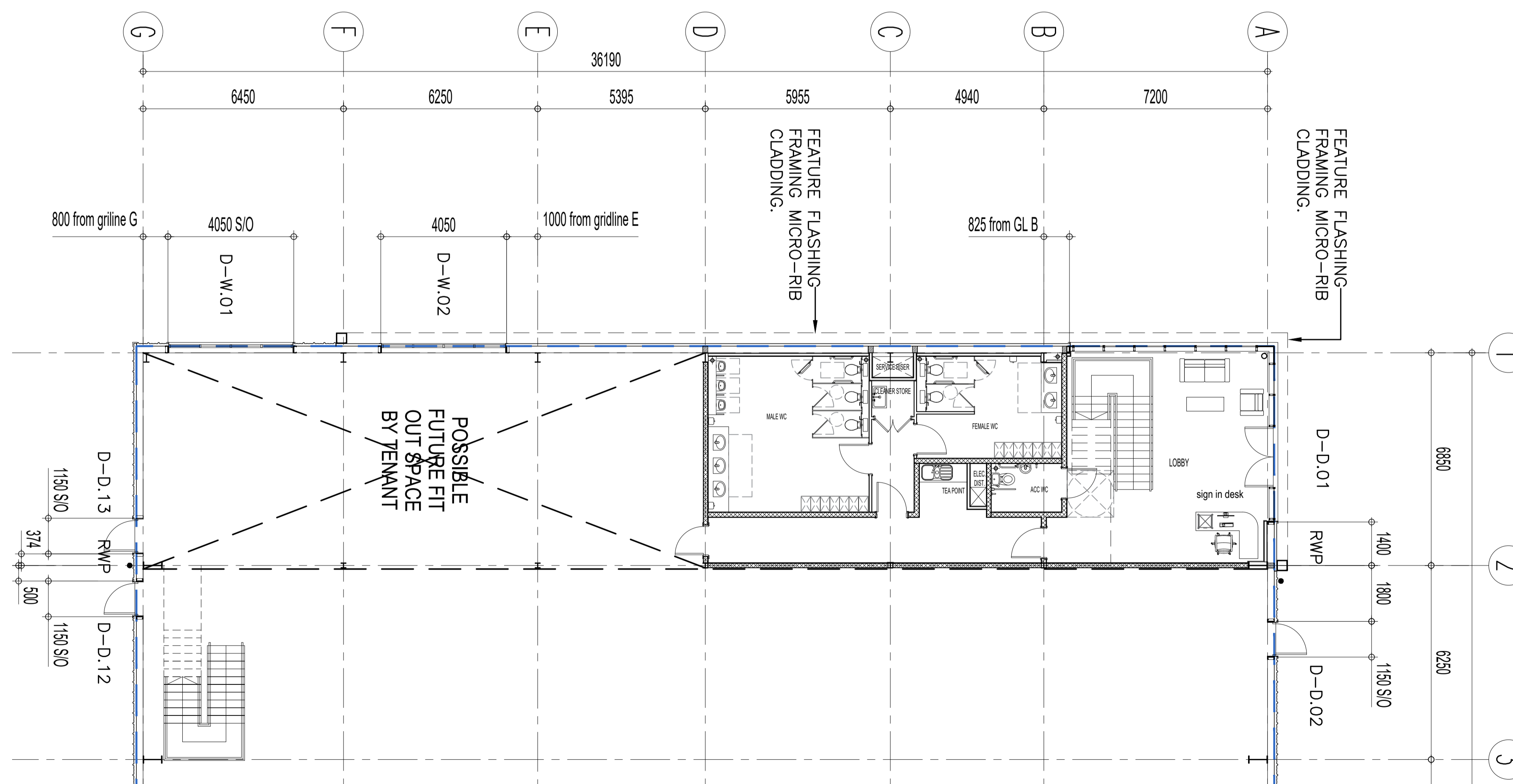
UNIT D - GROUND FLOOR OFFICE PLAN @ 1:100
