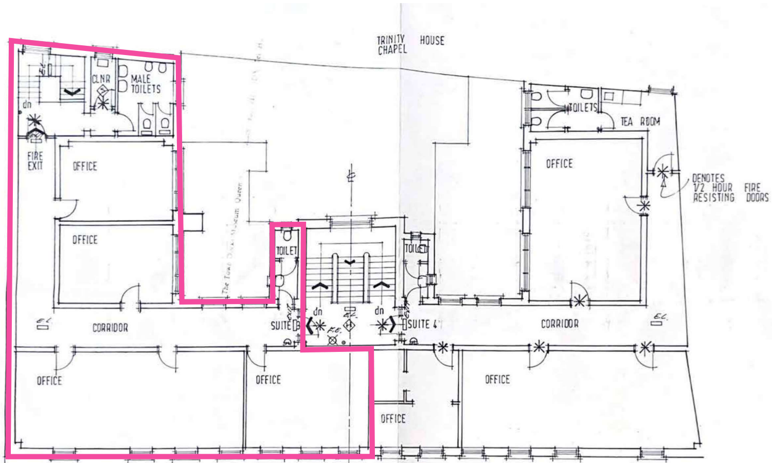
FIRST FLOOR PLAN - CARMELITE HOUSE
