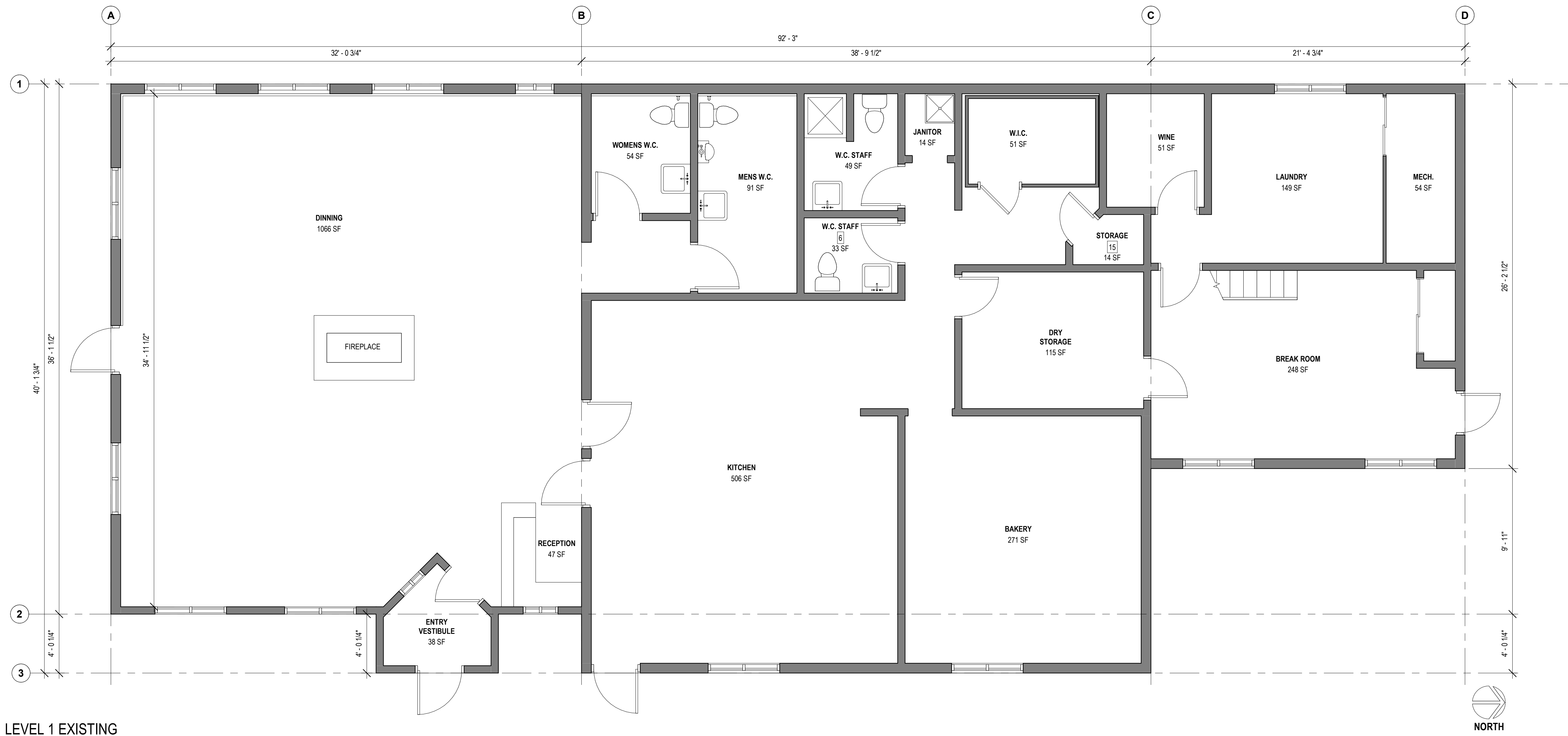
1 LEVEL 1 EXISTING 1/4" = 1'-0"
