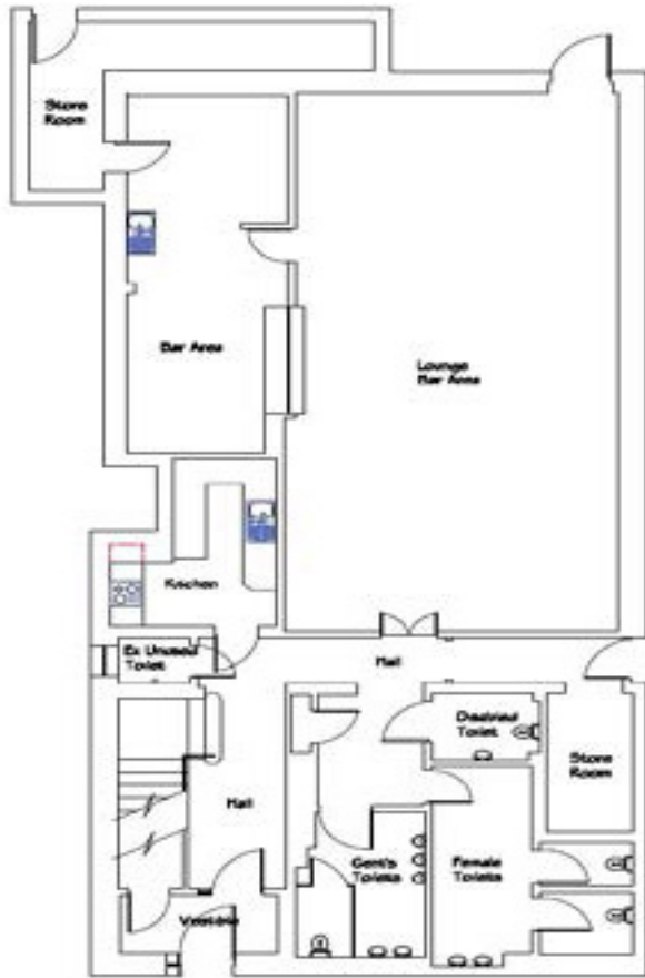
Existing Ground Floor Plan Scale 1:100
