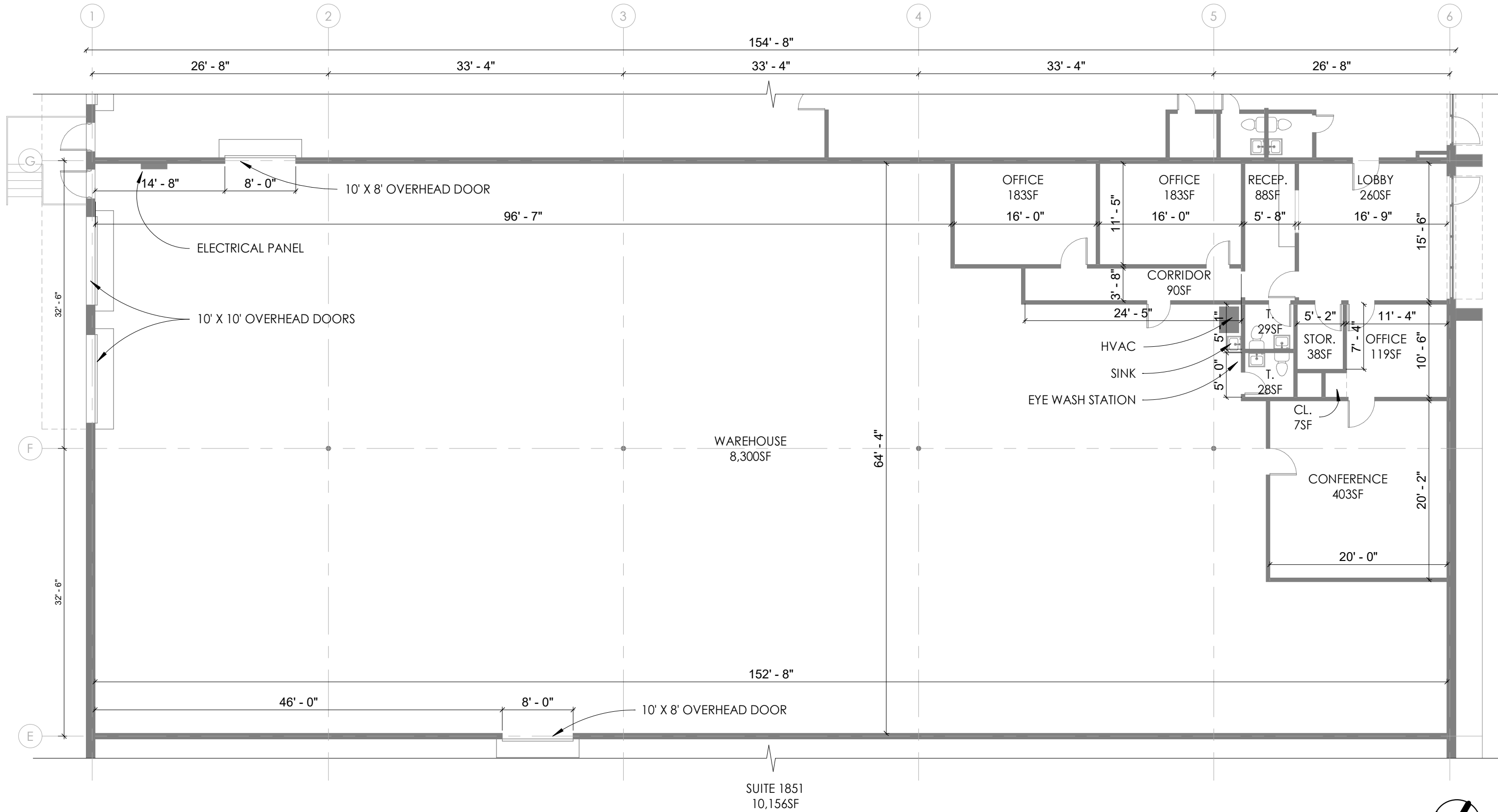
1 SUITE 1851 - EXISTING FLOOR PLAN 3/32" = 1'-0"
