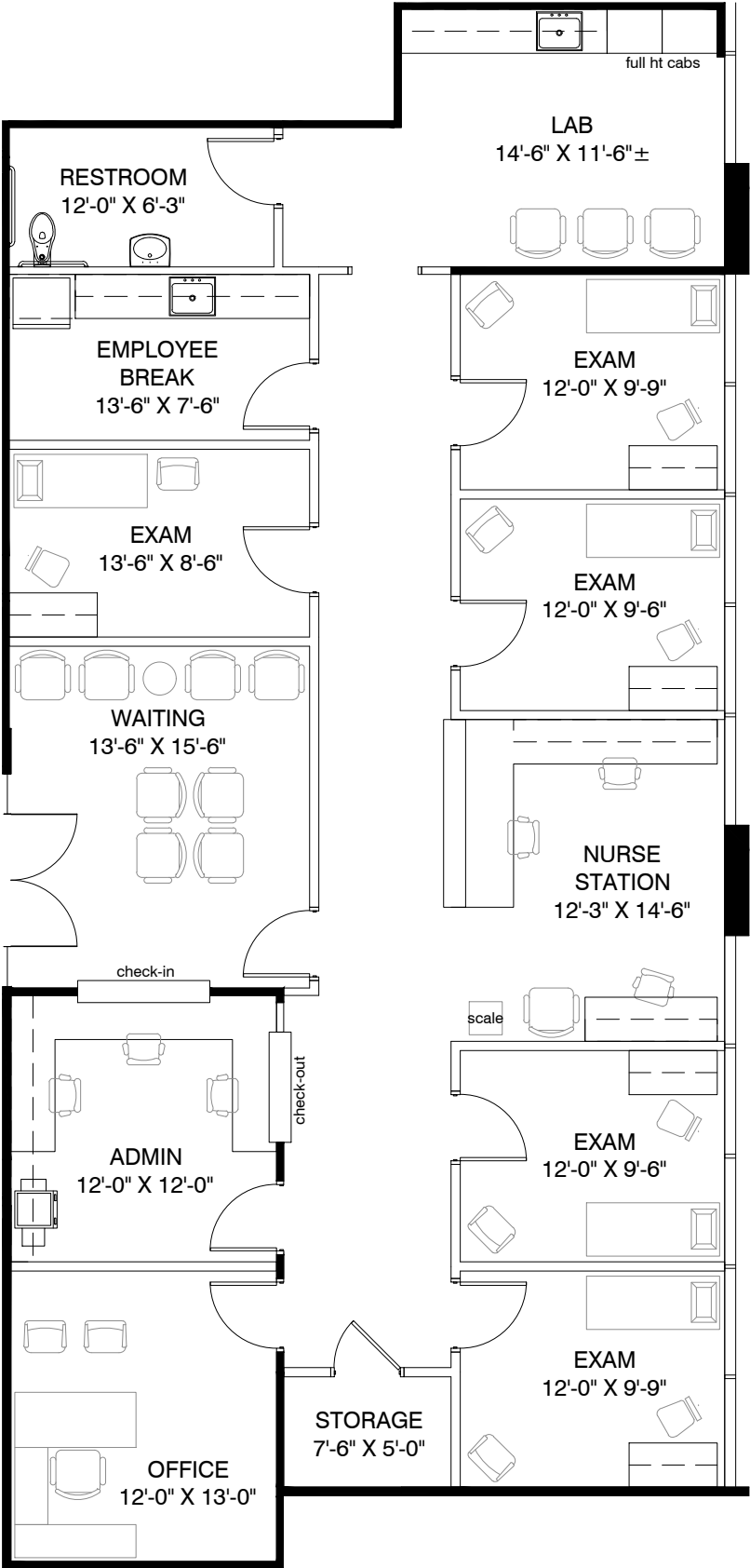
SUITE 100E / MEDICAL OFFICE CONCEPTUAL SUITE LAYOUT
