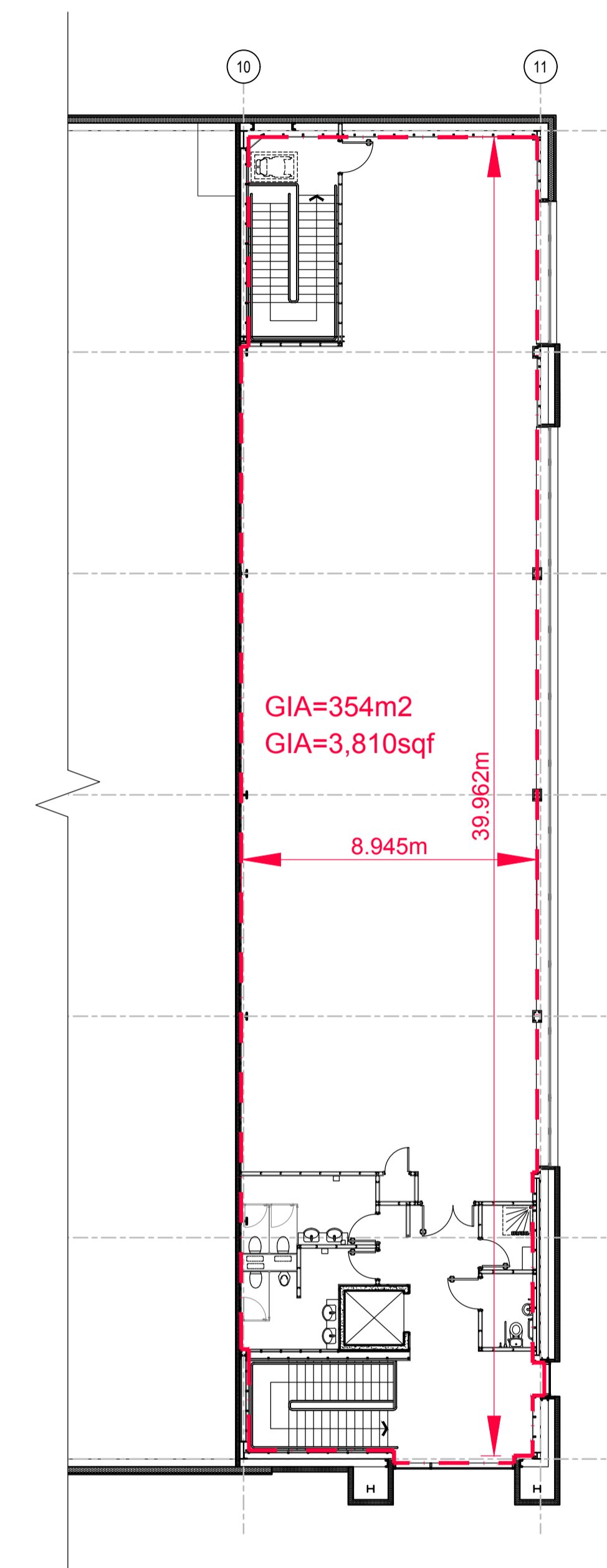
MEZZANINE PLAN
