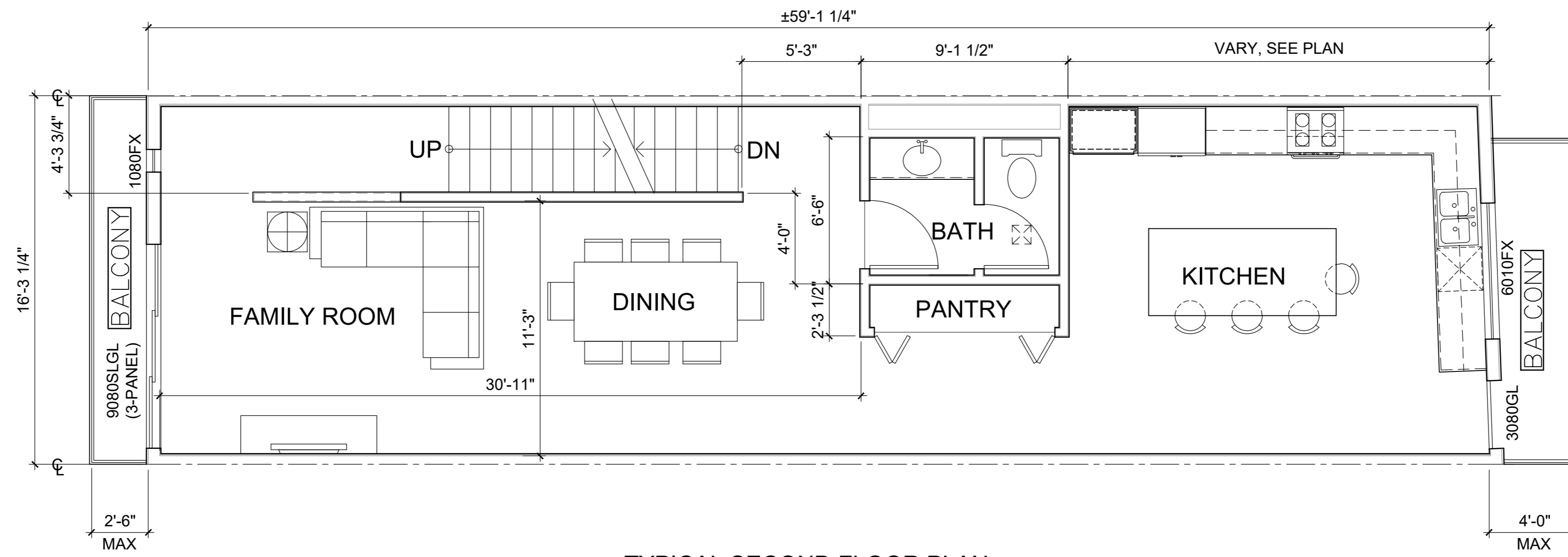
TYPICAL SECOND FLOOR PLAN
