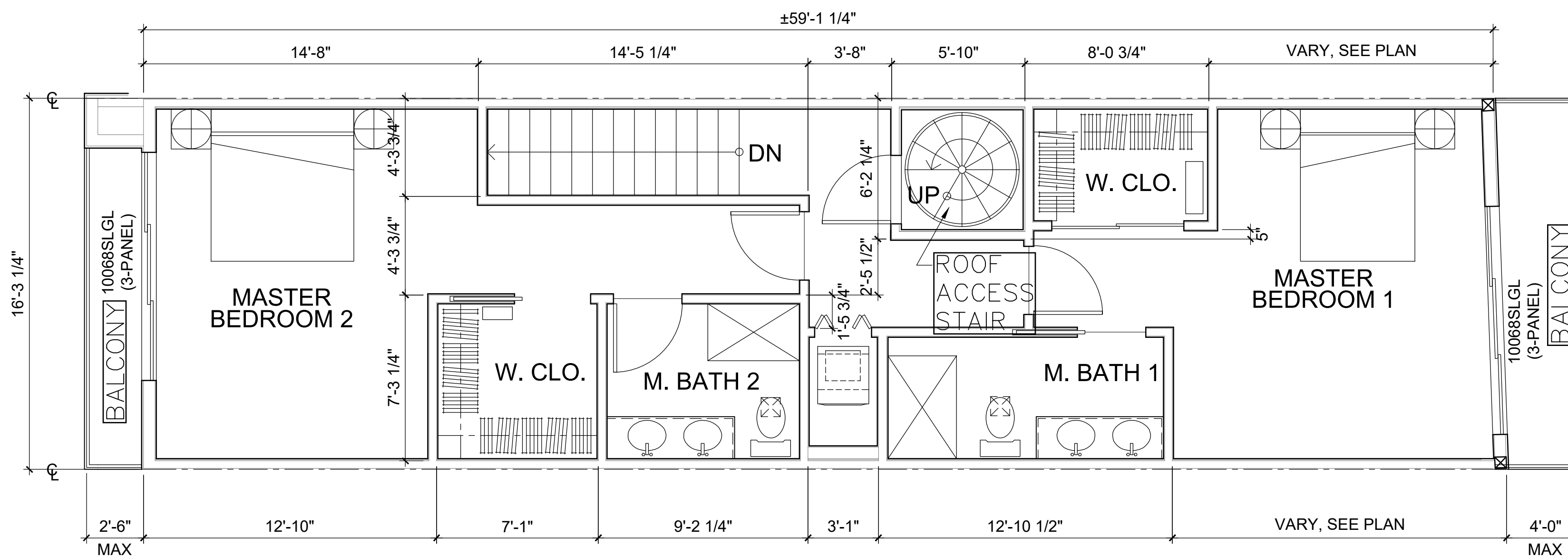
TYPICAL THIRD FLOOR PLAN
