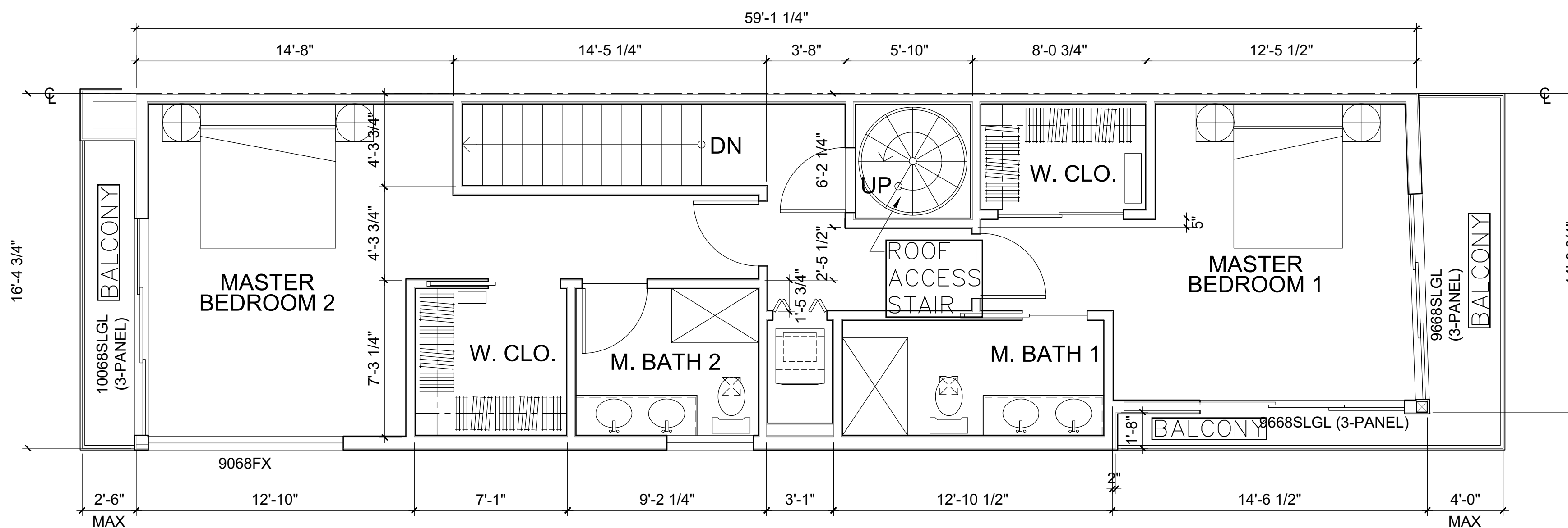
ALTERNATE THIRD FLOOR PLAN AT UNIT #5
