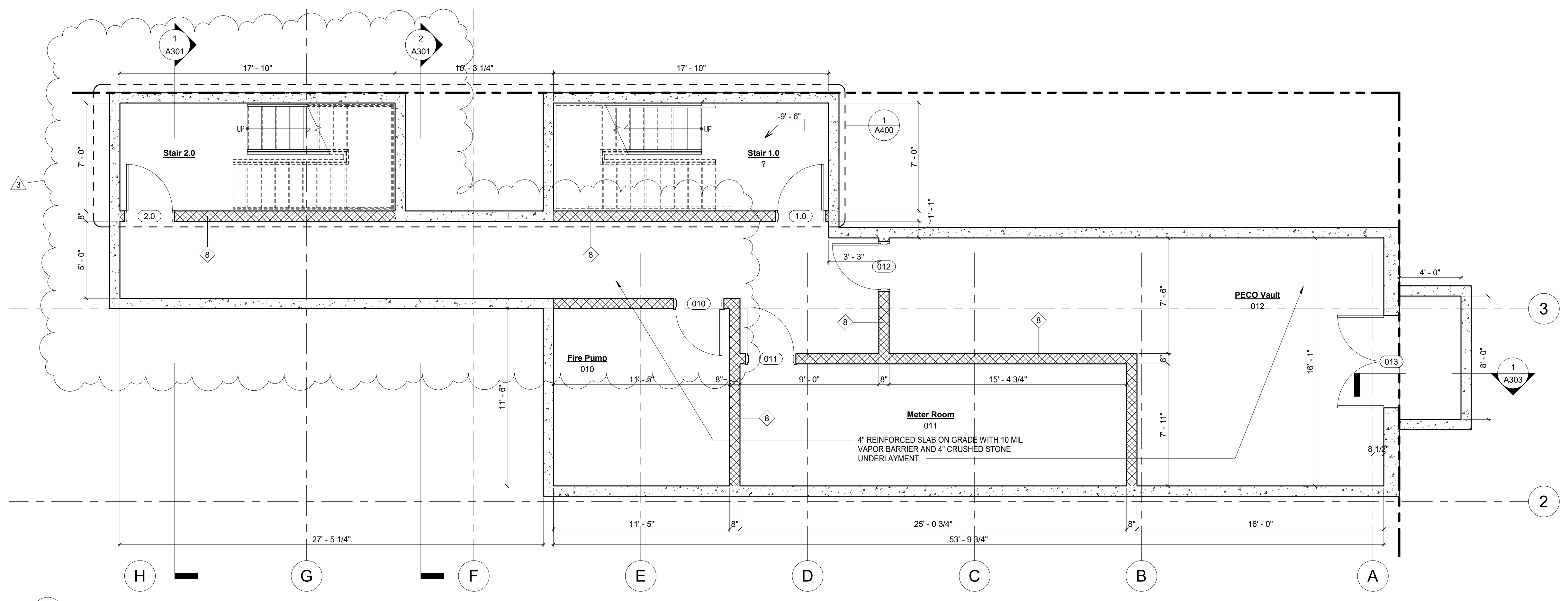
2 00 - BASEMENT PLAN A100 / 1/4" = 1'-0"
