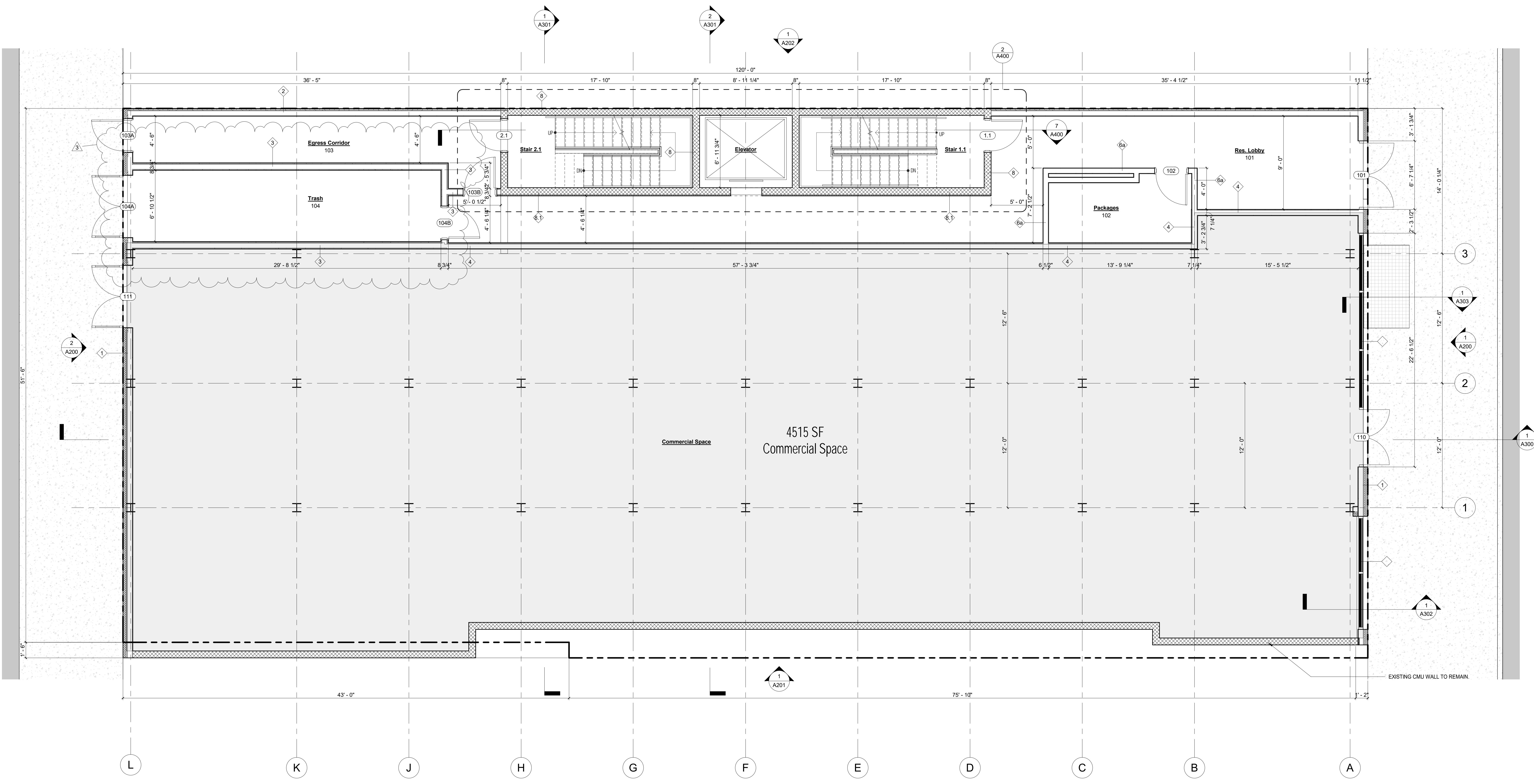
1 FIRST FLOOR PLAN A101 1/4" = 1'-0"
